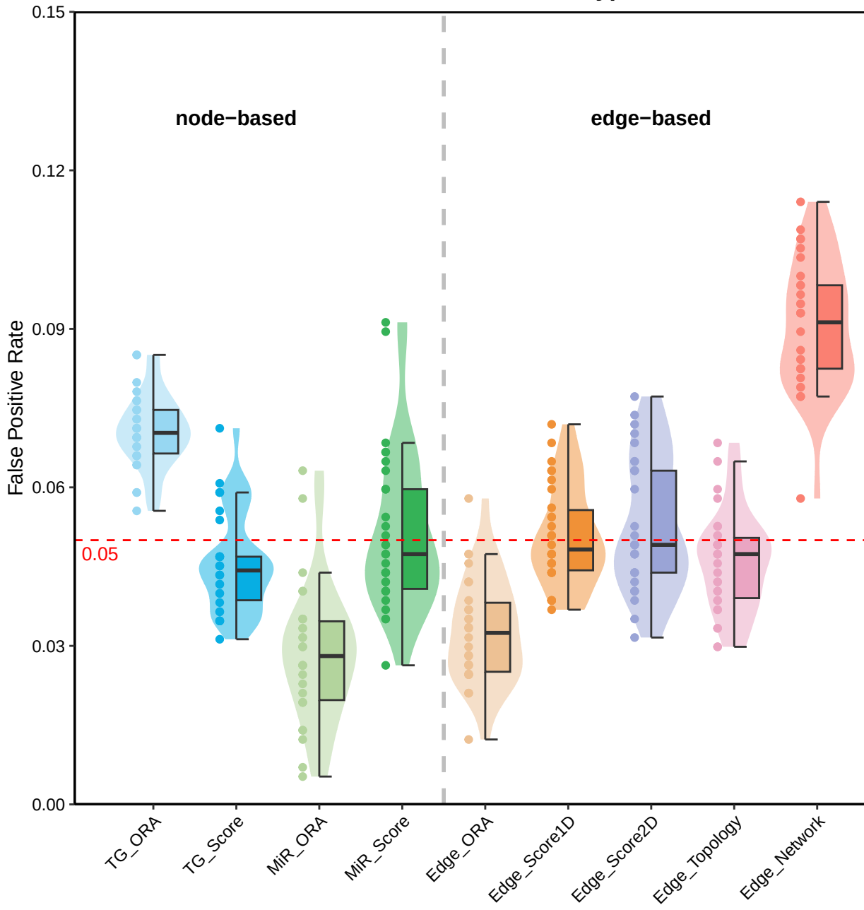
False Positive Rates Across 16 Cancer Types and 30 Seeds
