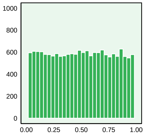
Edge_Score2D
