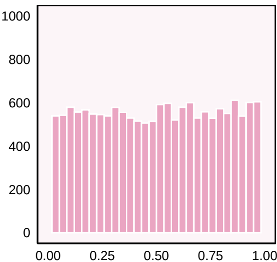
Edge_Topology
