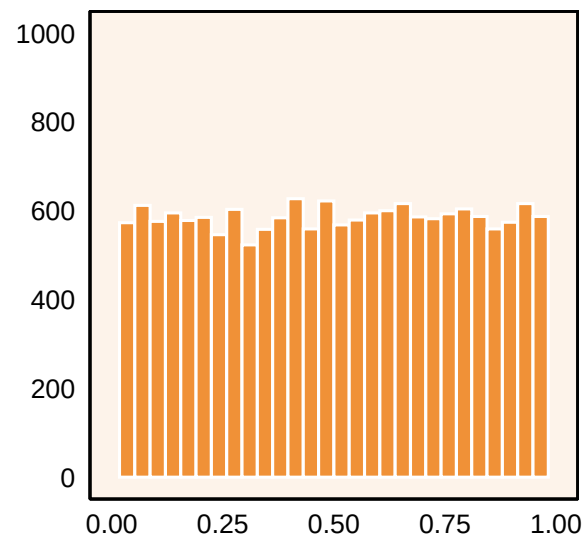
Edge_Network
