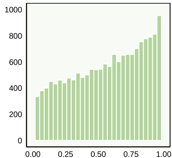
Edge_Score1D
