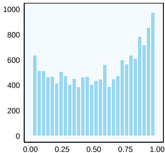
MiR_Score
