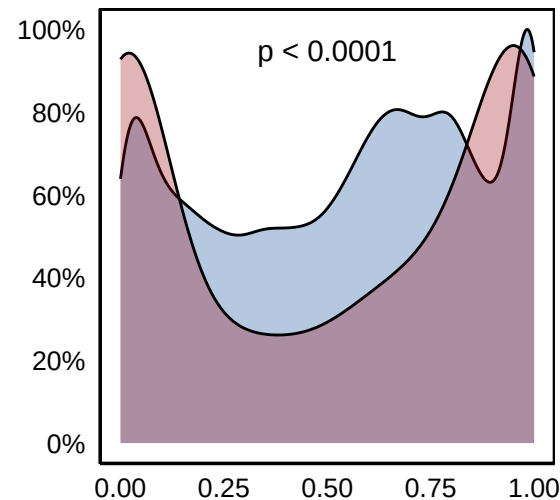
Edge_Network
