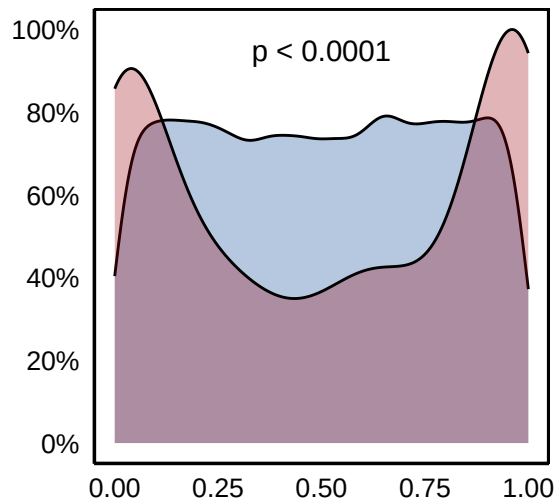
Edge_Score2D
