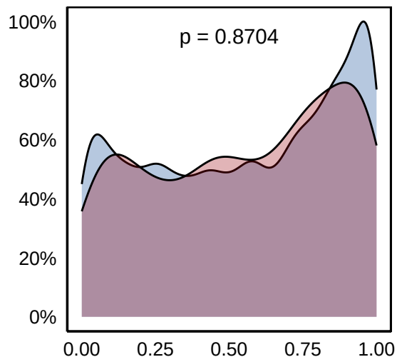
MiR_Score
