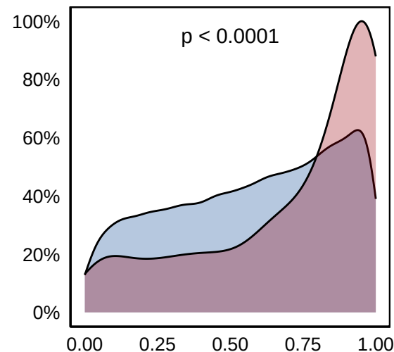
Edge_Score1D
