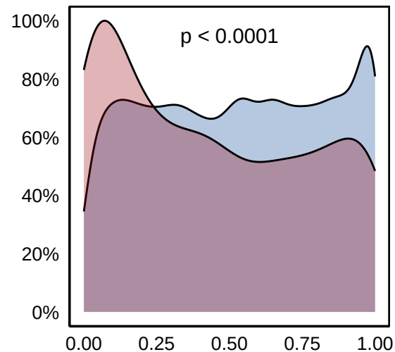
Edge_Topology
