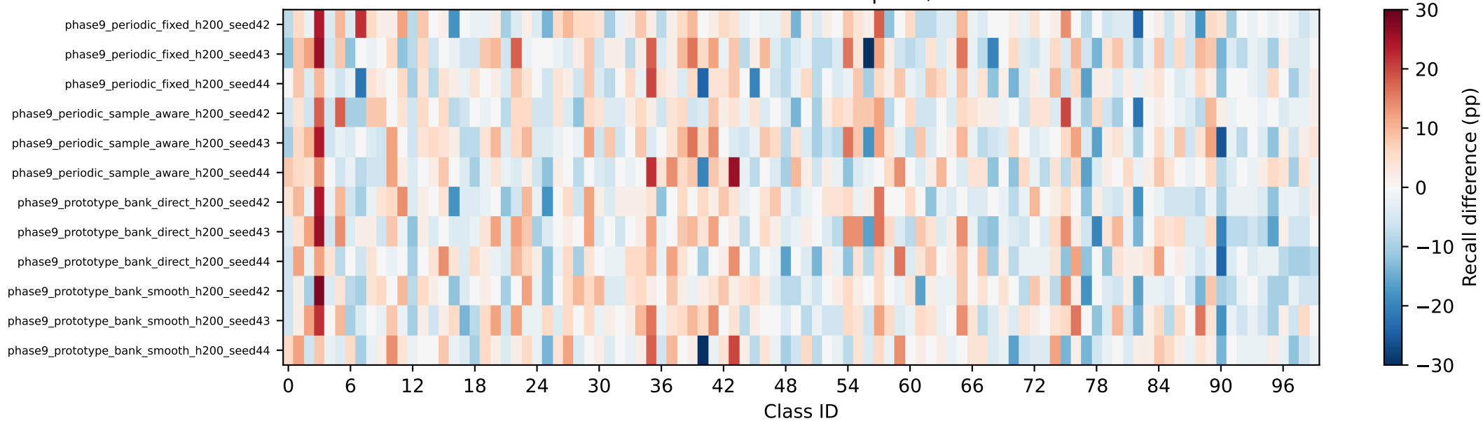
Per-seed recall difference | last, task 10
