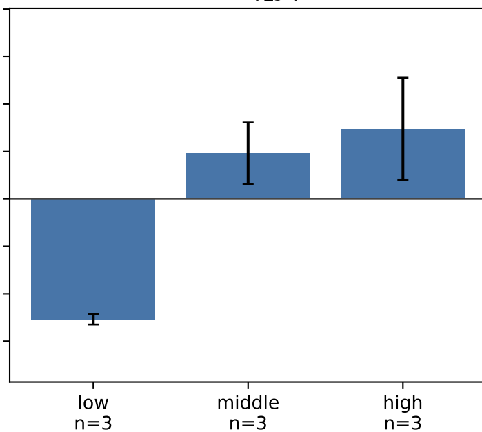
modality_gap
