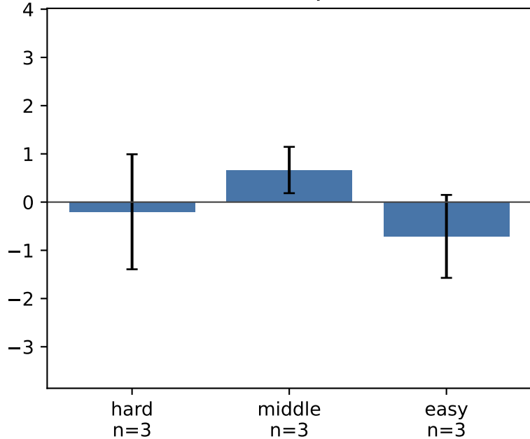
difficulty
