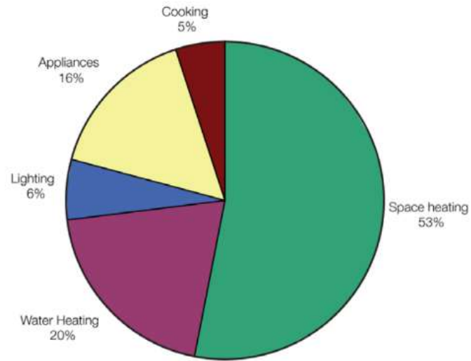
Figure 3 : Domestic Carbon Emissions – 2005, Source: (Department for communities and local government 2006)
