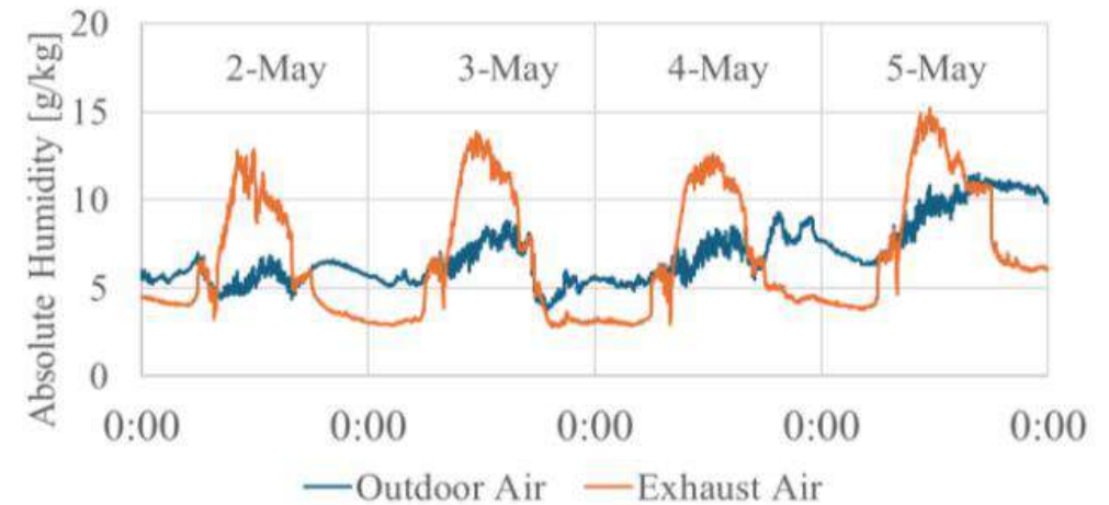
Fig. 7 Absolute Humidity over high solar irradiance days.
