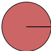
Bacterial_DNA_D4
