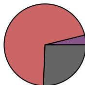
Bacterial_DNA_D5
