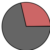
Bacterial_DNA_D6
