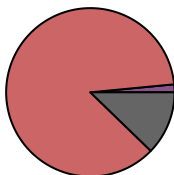
Bacterial_DNA_D8
