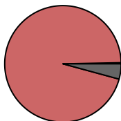
Bacterial_DNA_D7
