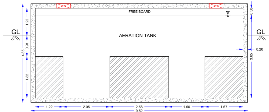
CROSS SECTION ALONG A - A
