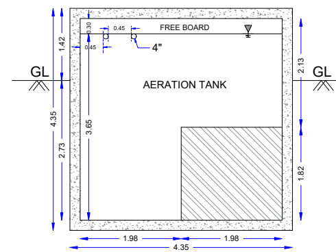
CROSS SECTION ALONG B - B
