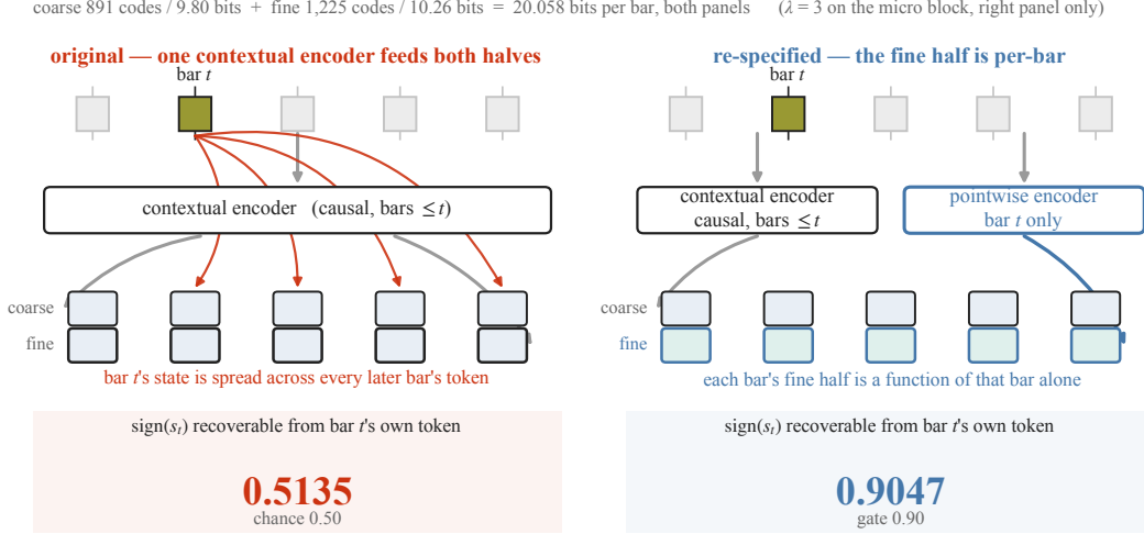
Figure 1: One interface change decides whether a microstructure signal survives tokenization. Each bar is encoded to a token pair — a coarse and a fine subtoken, together 20.058 bits — which is what the autoregressive stage consumes. Left, the original design: a single causal encoder produces both halves. Because that encoder is contextual, bar t 's own state is distributed across the tokens of every later bar in the window, so the window reconstructs while the per-bar symbol carries almost nothing: the sign of bar t 's microstructure state is recoverable from bar t 's own token at 0.5135, against a chance rate of 0.50. Right, the re-specified design: the fine half is produced by a pointwise encoder that sees only the current bar, shaped by a per-bar bottleneck objective that weights the microstructure block as a class. Recoverability rises to 0.9047 and is enforced thereafter by a gate at 0.90. Bits per bar, the vocabulary split, the backbone and every evaluation instrument are identical between the two panels, so per-bar legibility is the only quantity that differs. What that difference buys downstream — the same planted signal recovered on the right and not on the left — is Figure 3; this panel is the interface, not the result.
