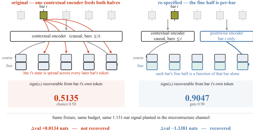
Figure 1: One interface change decides whether a microstructure signal survives tokenization. Each bar is encoded to a token pair — a coarse and a fine subtoken, together 20.058 bits — which is what the autoregressive stage consumes. Left, the original design: a single causal encoder produces both halves. Because that encoder is contextual, bar t 's own state is distributed across the tokens of every later bar in the window, so the window reconstructs while the per-bar symbol carries almost nothing: the sign of bar t 's microstructure state is recoverable from bar t 's own token at 0.5135, against a chance rate of 0.50. Right, the re-specified design: the fine half is produced by a pointwise encoder that sees only the current bar, shaped by a per-bar bottleneck objective that weights the microstructure block as a class. Recoverability rises to 0.9047 and is enforced thereafter by a gate at 0.90. Bits per bar, the vocabulary split, the backbone and every evaluation instrument are identical between the two panels. Below: the same fixture, the same training budget and the same 1.151-nat signal planted in the microstructure channel, before and after — the planted arm ends 0.0134 nats worse than its matched control on the left, and 1.3381 nats better on the right.
