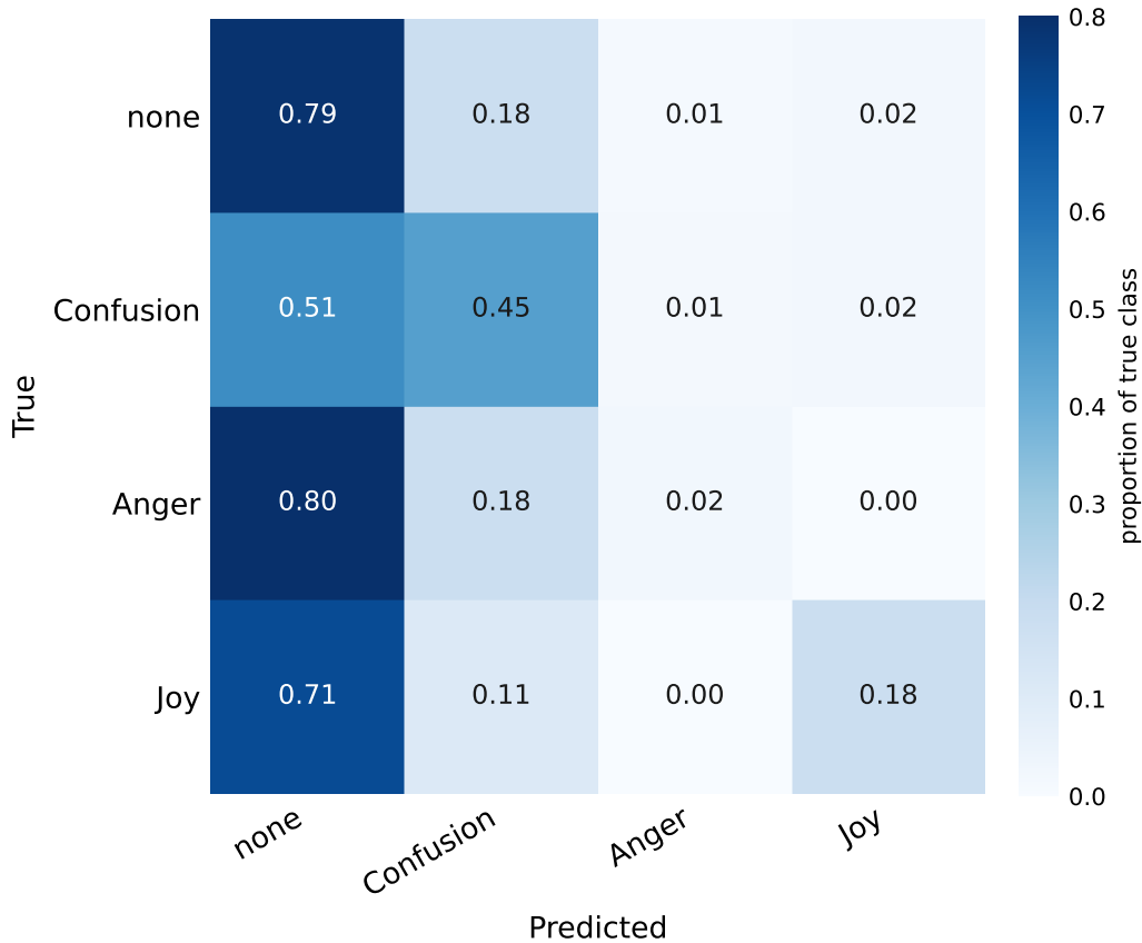
DUX human annotation, 4-class - fused
