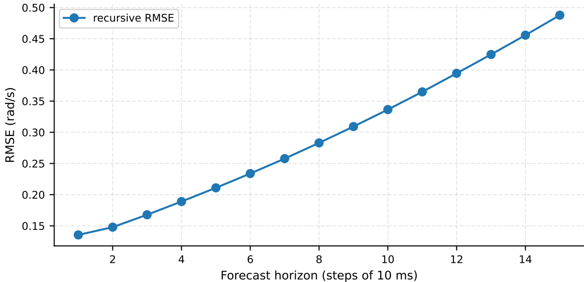
Fig. 2 — Main LSTM recursive multi-step RMSE (frozen test metrics)
