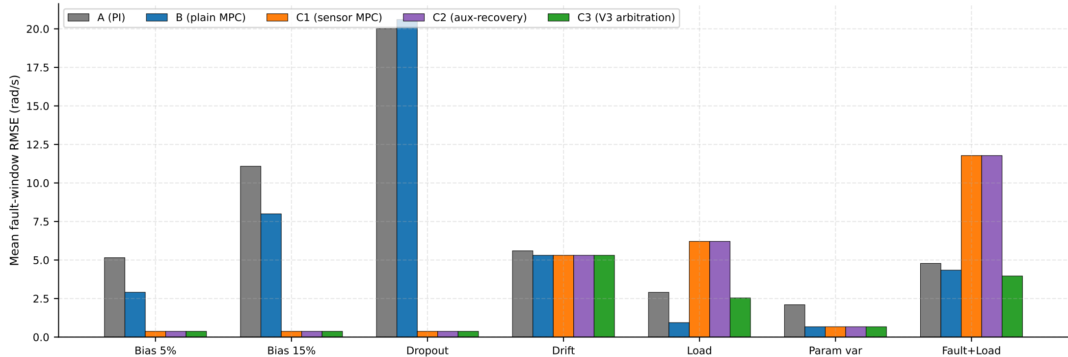
Fig. 4 — V3 frozen holdout: fault-window RMSE by scenario and controller (mean of 5 seeds)
