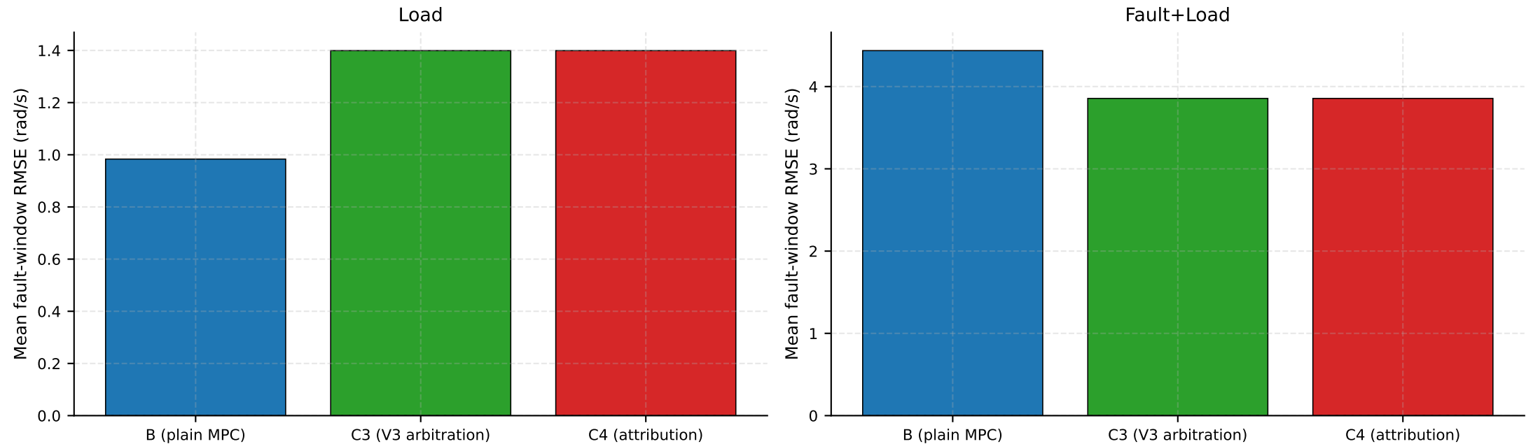
Fig. 6 — C4 development: C4 adds nothing over C3 (mean of 5 dev seeds)
