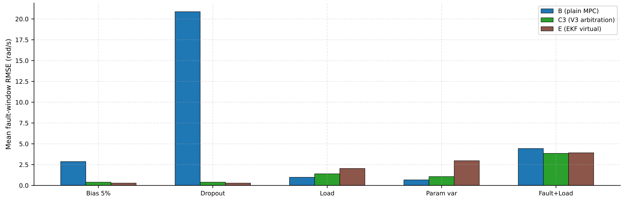
Fig. 7 — EKF comparator grid: E vs B vs C3 (mean of 5 dev seeds)
