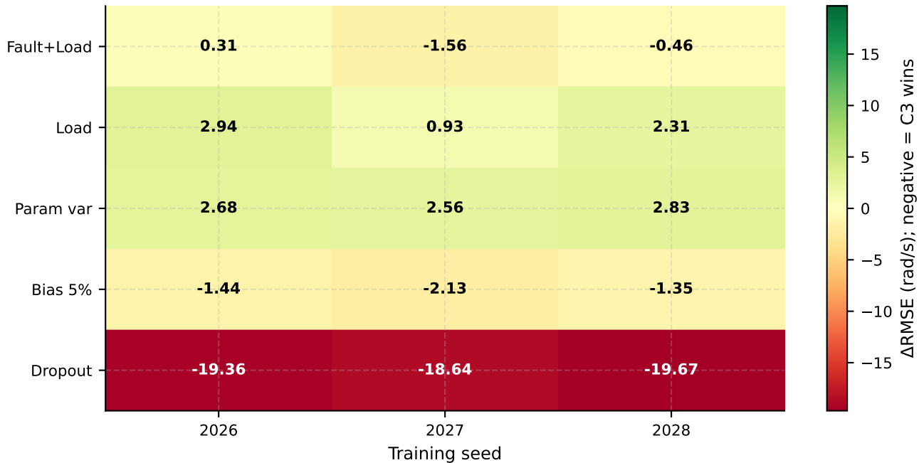
Fig. 8 — Mean paired C3–B \Delta RMSE (rad/s) by scenario \times training seed
