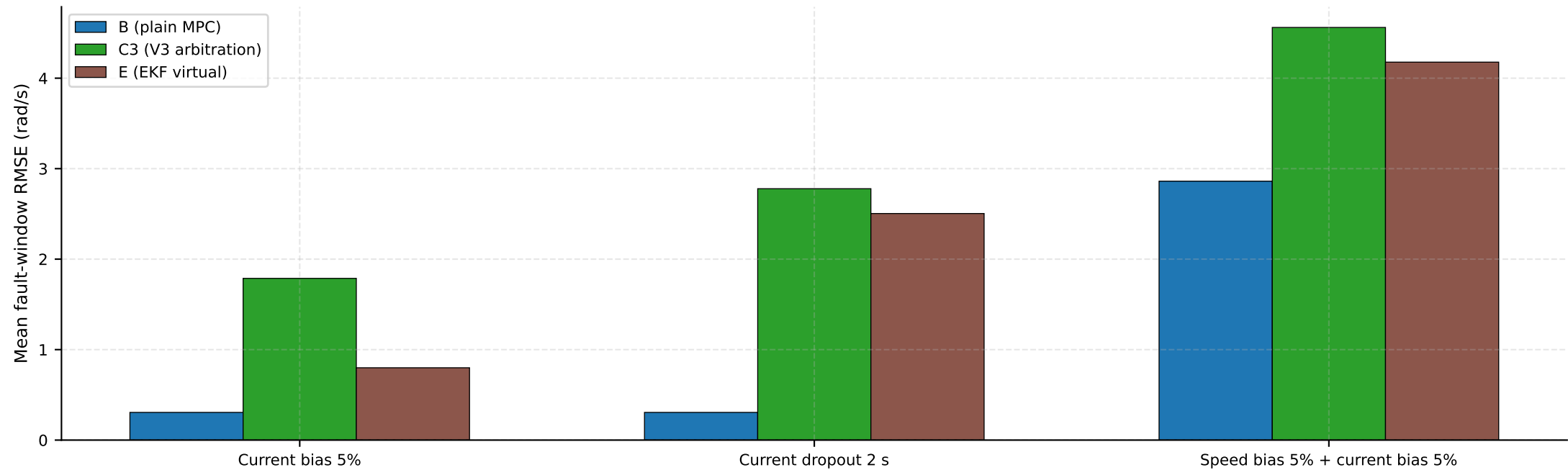
Fig. 12 — Current-sensor boundary: B/C3/E under current-channel corruption
