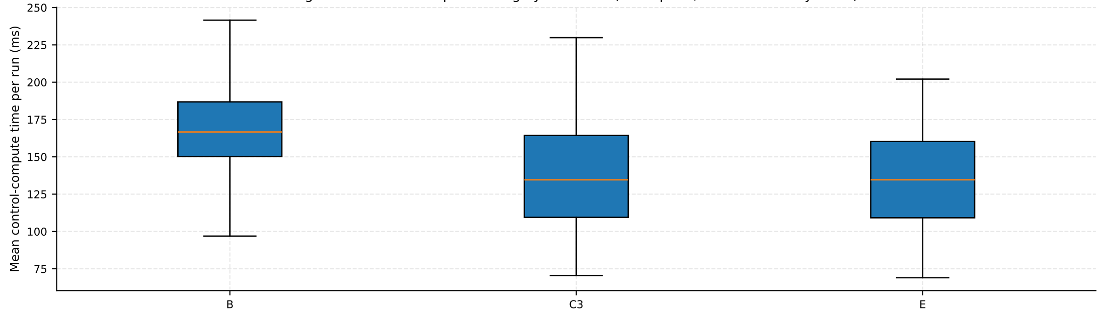
Fig. 13 — Control-compute timing by controller (descriptive; NOT a feasibility claim)
