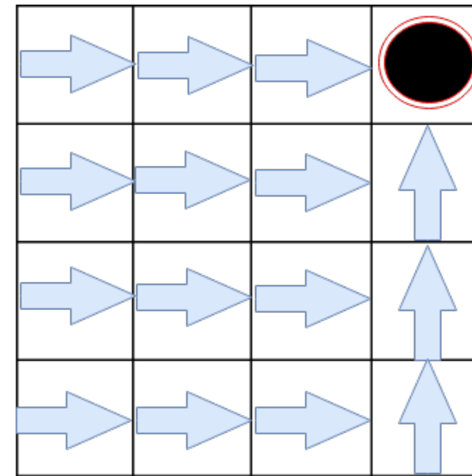
Target Policy
