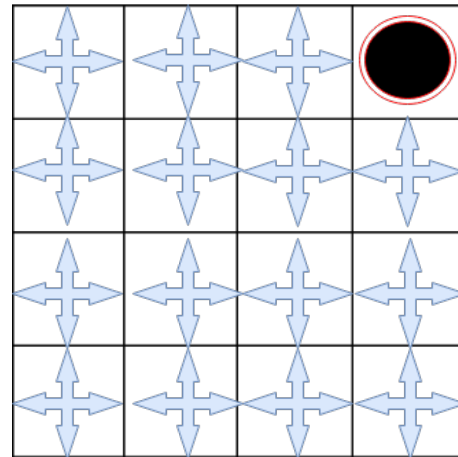
Behavior Policy
