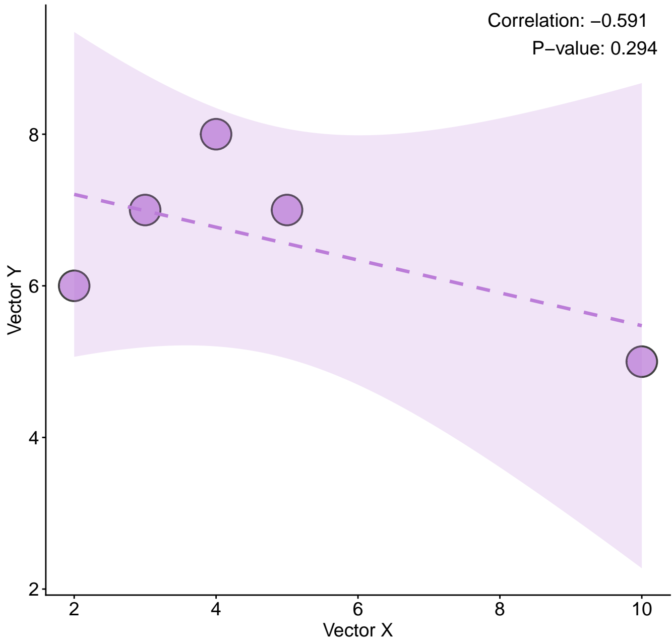
Correlation Plot
