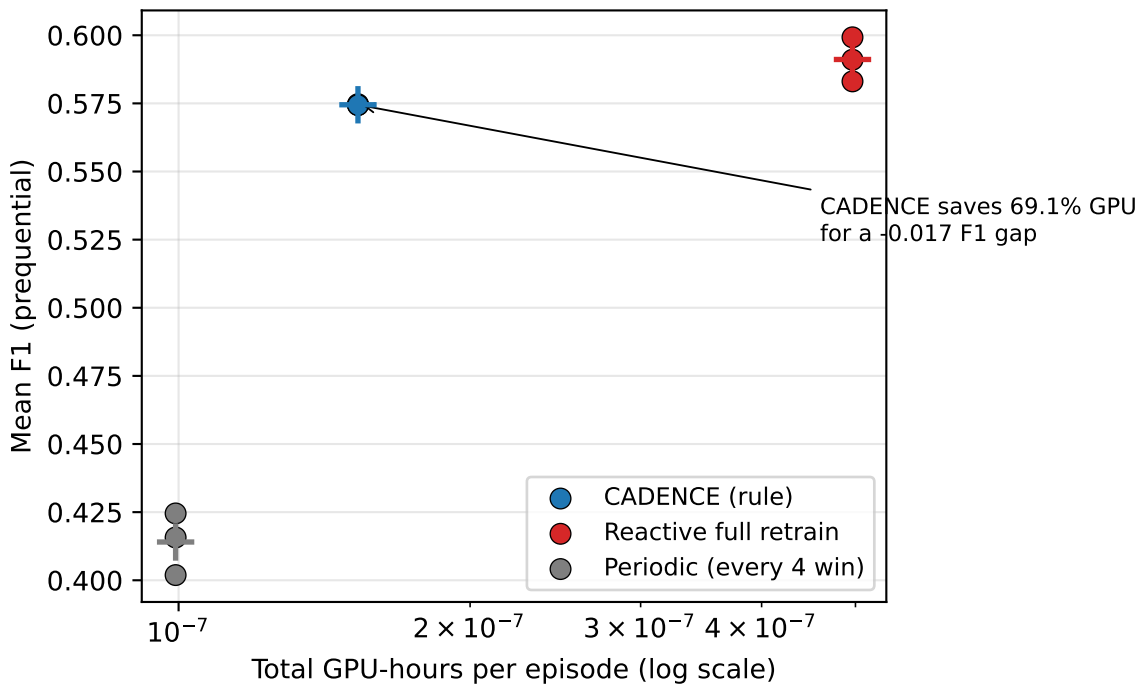
Elec2 real-drift end-to-end: Pareto frontier (3 seeds; + = mean)
