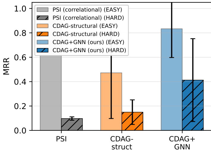
MRR
