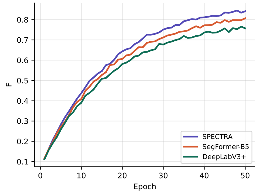
Validation F-score ( \beta^2=0.3 )
