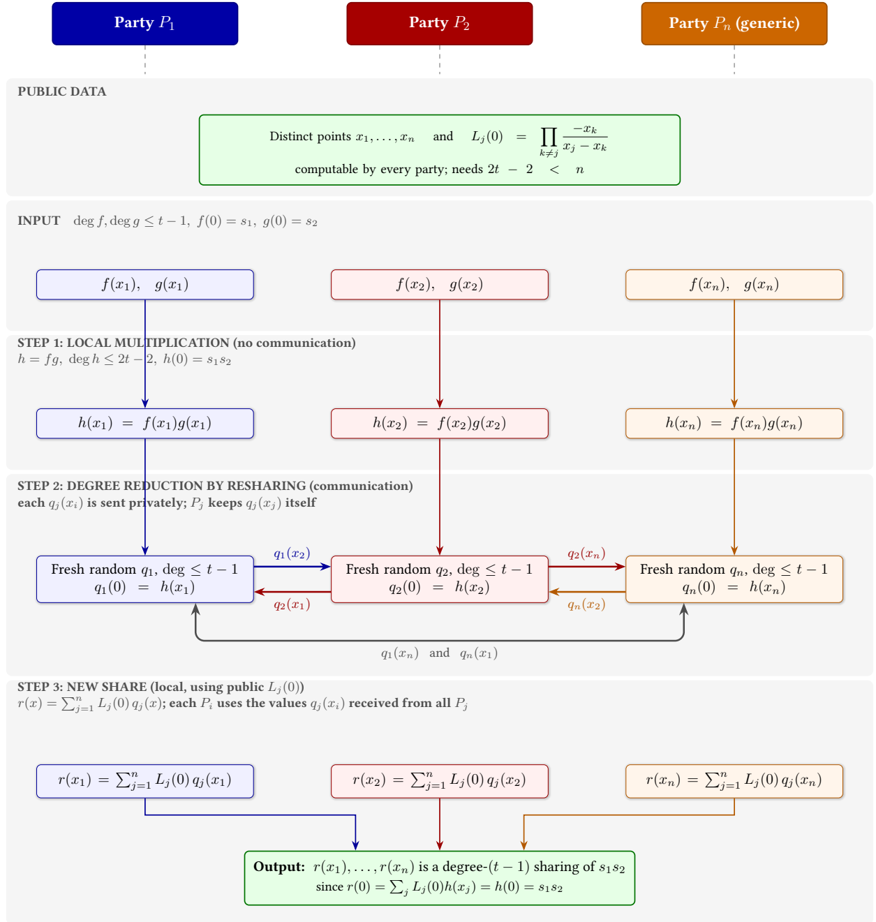
Figure 1: Multiplication of Shamir-shared secrets s_1 and s_2 with sharing polynomials f, g of degree t - 1 .
