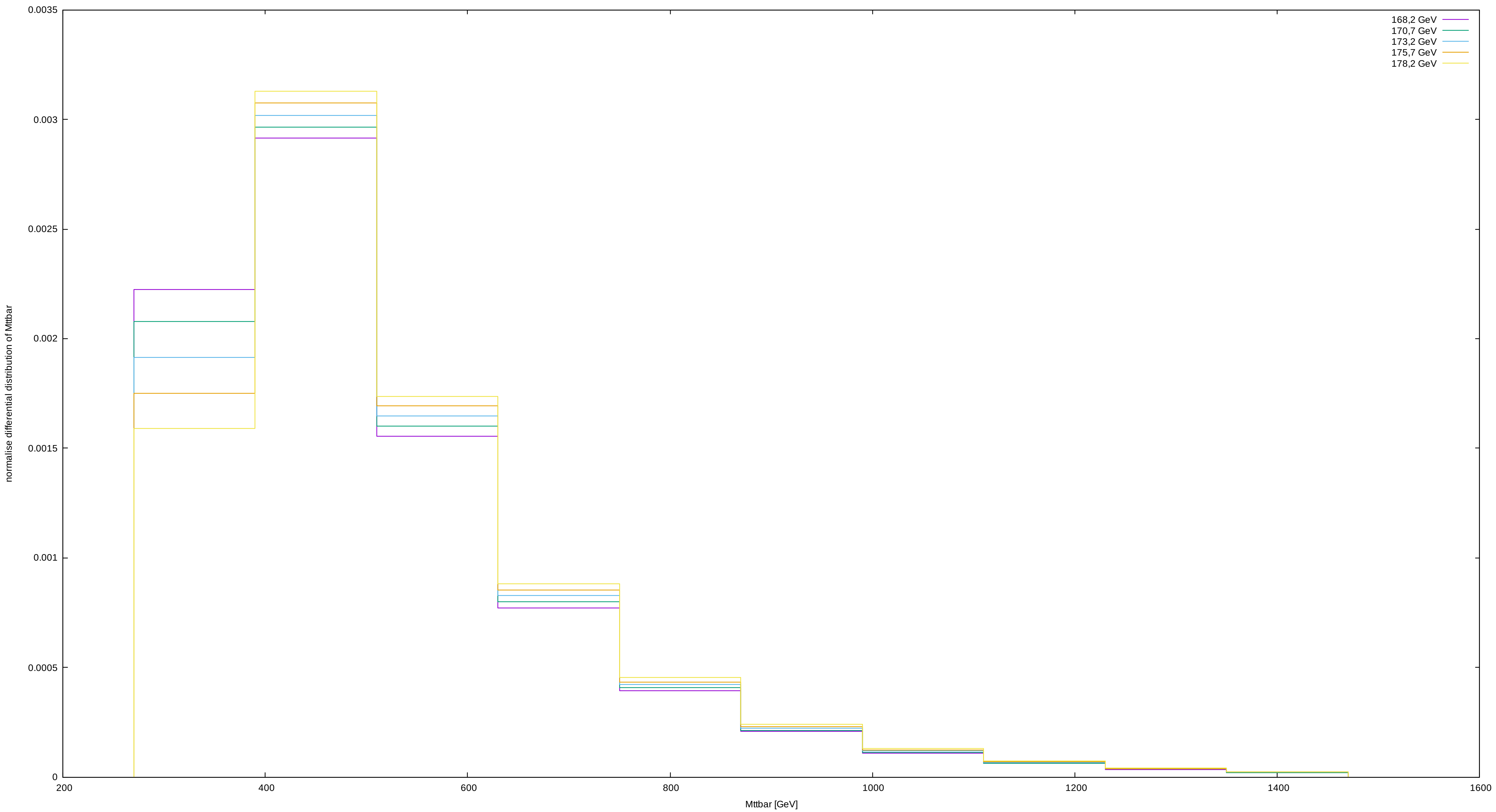
Comparison of differential distribution of Mttbar for 5 different masses in Et/2 scale
