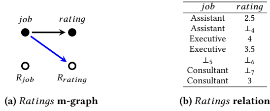
Figure 6: Ratings relation and its m-graph
