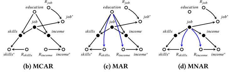
Figure 1: An augmented relation and some possible m-graphs. Solid nodes represent incomplete attributes. Starred nodes represent their proxy attributes. The other hollow nodes represent complete attributes and missingness mechanisms. Blue edges into missingness mechanisms R indicate the cause of missingness.
