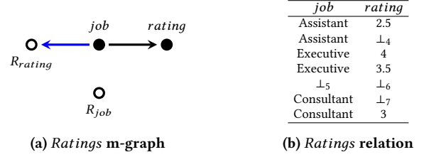
Figure 6: Ratings relation and its m-graph
