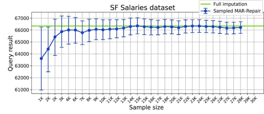
Figure 8: Sampled MAR-Repair convergence on SF Salaries.
