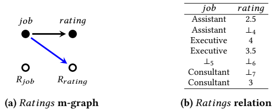
Figure 7: Ratings relation and its m-graph, used in Example D.1.
