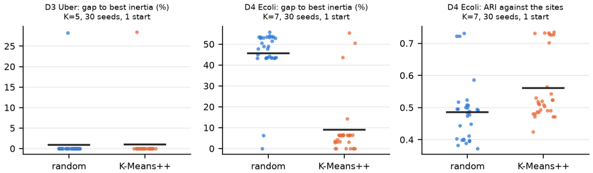
Figure 5: Ablation A, one dot per seed (30 per start method); bars mark the mean. Left and centre: inertia above the best run on D3 and D4. Right: ARI on D4. K-Means++ moves most D4 starts near the best inertia, and reaches the high-ARI group (about 0.73) in 8 of 30 seeds against 3 of 30 for random starts. Cause: spreading the starting centres out makes a good local optimum more likely, not certain.
