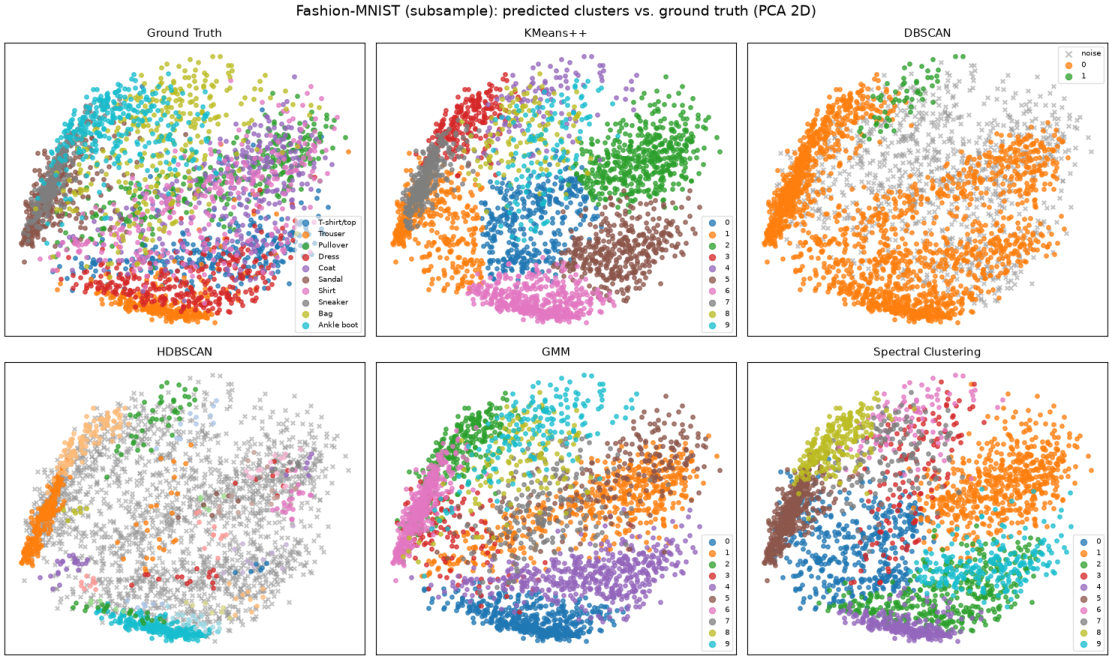
Figure 13: D5 Fashion-MNIST (3,000 images; clustered in 50 PCA dimensions, plotted in the first two). DBSCAN merges most classes into one cluster (ARI 0.03); HDBSCAN calls 71% of points noise (ARI 0.05). Spectral, GMM and K-Means++ reach ARI 0.40, 0.39, 0.34.
