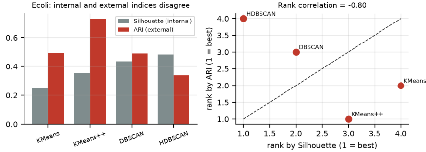
Figure 4: D4, silhouette against ARI for the four methods at each method’s best-ARI setting. Left: the two scores. Right: their ranks; points on the dashed line would mean the two agree. The silhouette ranks the methods almost in reverse (Spearman \rho = -0.80 ); the same holds at the settings chosen without labels (Table 4). Cause: the silhouette ignores noise and favours compact clusters.
