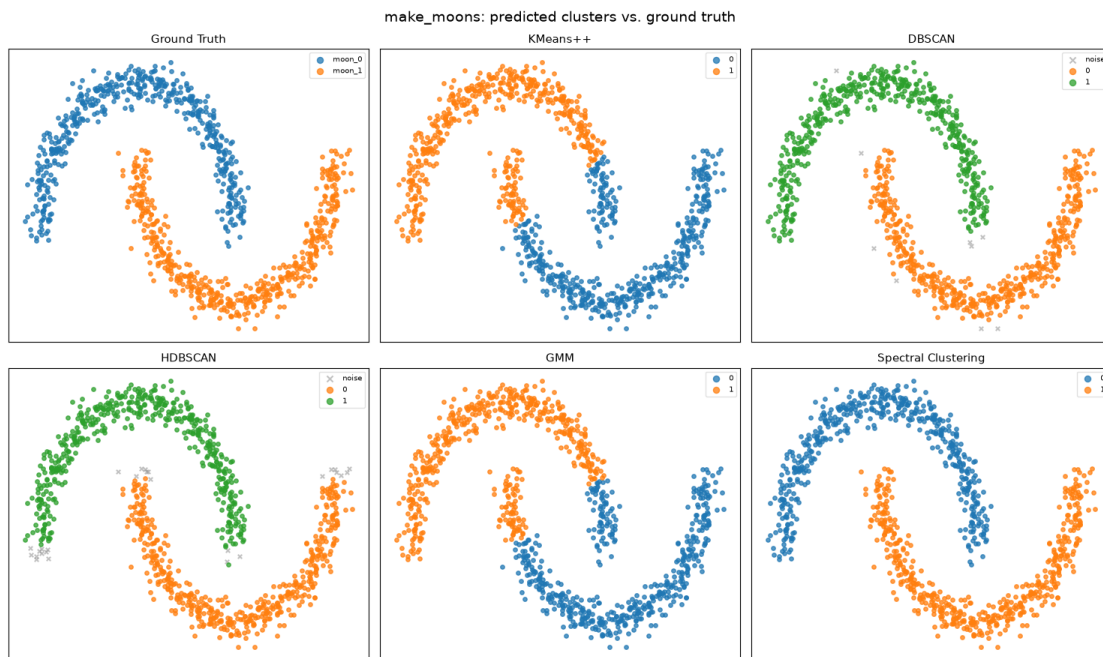
Figure 10: D1 make_moons. K-Means++ and GMM cut both moons with a straight boundary (ARI 0.48, 0.49); DBSCAN, HDBSCAN and Spectral follow the curves (ARI 0.98, 0.95, 1.00). Grey crosses: noise.
