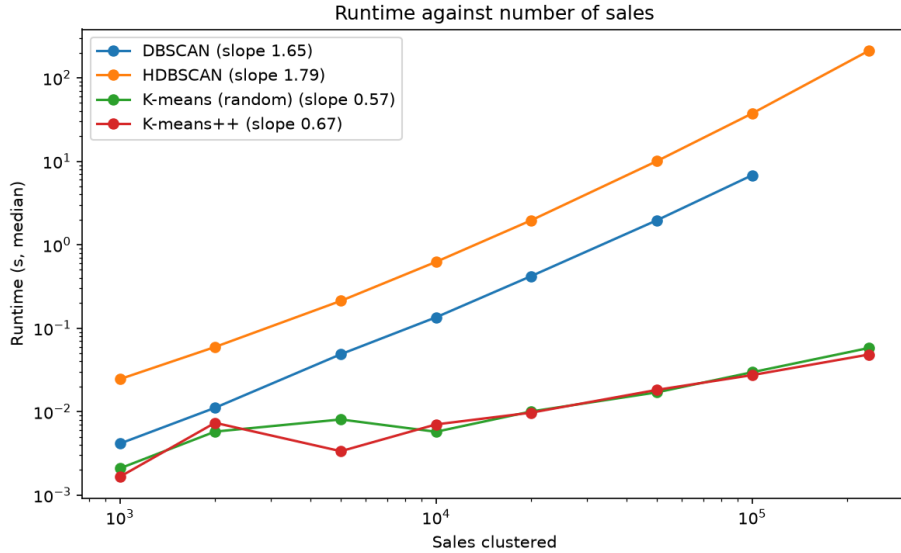
Figure 9: D8, median fit time against the number of sales, log-log, at the chosen settings; the slope of each line is in the legend. DBSCAN stops at 100,000 sales: the full data would need about 6 GB of neighbour indices.
