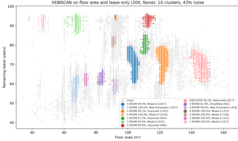
Figure 11: D8, success of HDBSCAN on floor area and remaining lease only ( min_cluster_size 200; grey: noise). Each cluster is one standard flat design; the legend gives its main flat type and model. Cause of success: fixed building plans create real dense spots in these two features.
