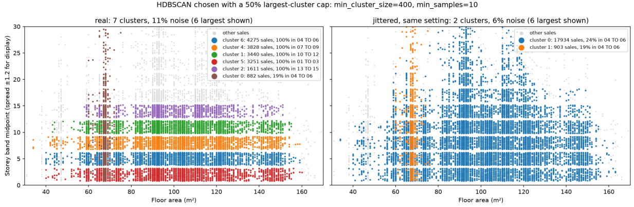
Figure 8: D8, HDBSCAN chosen under a 50% largest-cluster cap. Left, recorded values: 6 of 7 clusters are single storey bands. Right, the same setting on jittered values: 2 clusters. Cause: storeys recorded in 3-storey bands create exact ties that density methods read as dense regions.
