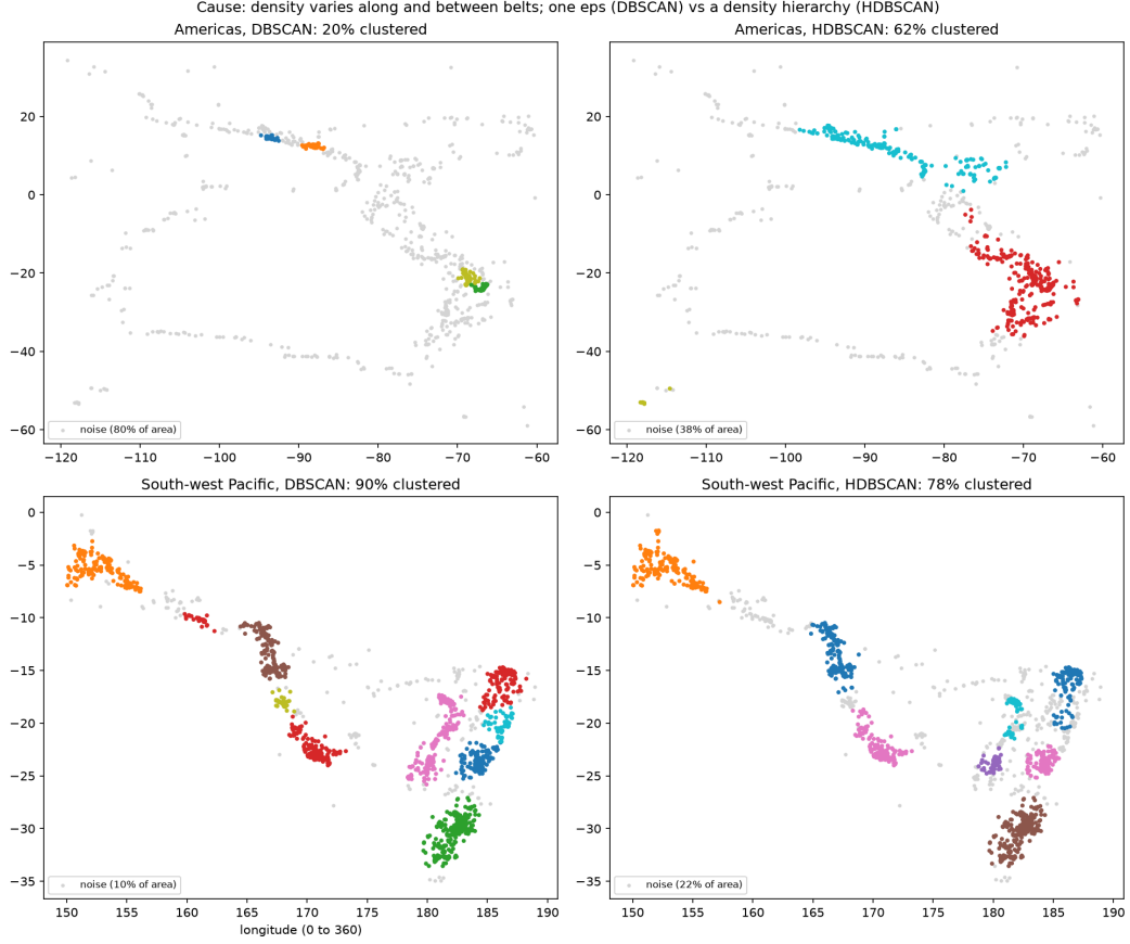
Figure 2: D2, DBSCAN ( \varepsilon = 101.8 km) against HDBSCAN in a sparse region (top, the Americas) and a dense one (bottom, the south-west Pacific); grey points are noise. Success of HDBSCAN on the sparse belts, at the cost of trimming the dense ones. Cause: density varies along and between belts.
