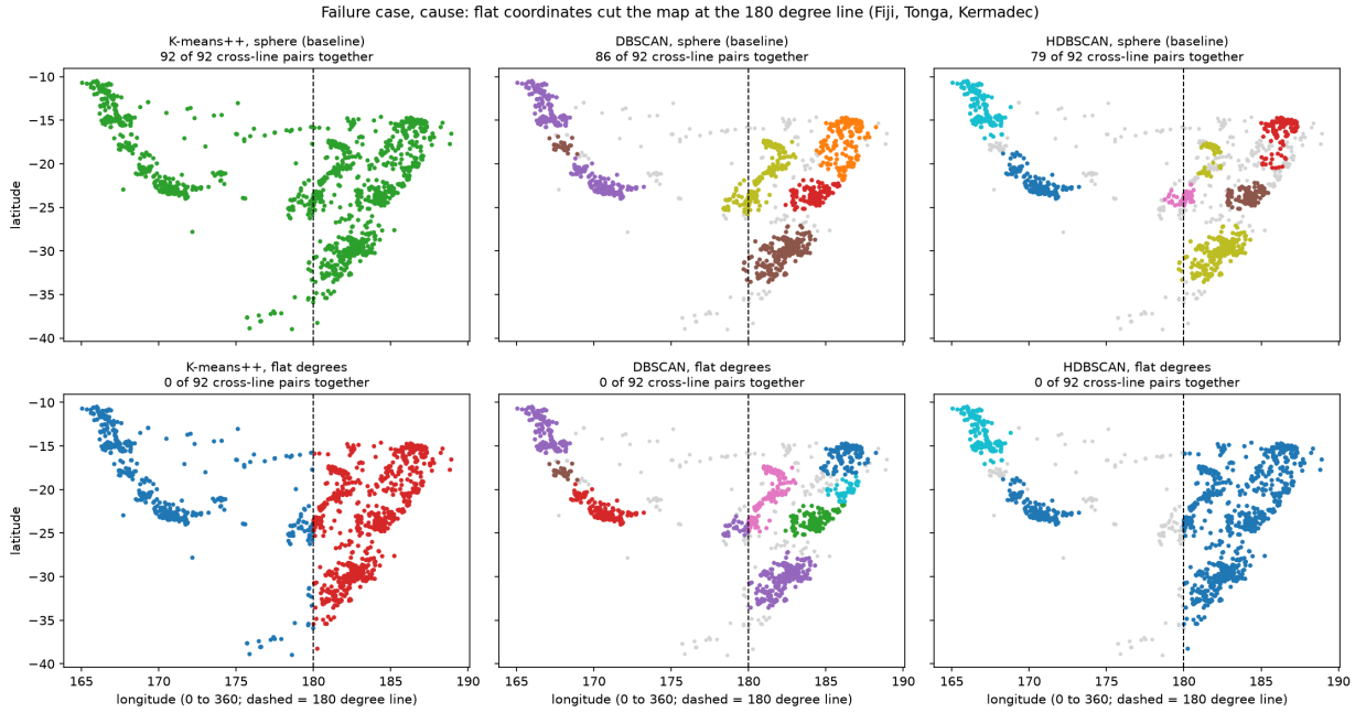
Figure 6: Fiji, Tonga and Kermadec, drawn on longitudes 0 to 360° (dashed: the 180° meridian). Top: on the sphere, clusters cross the line. Bottom: on flat degrees, every method splits the system at the line. Cause: flat coordinates treat 179.9°E and 179.9°W as 359.8° apart.
