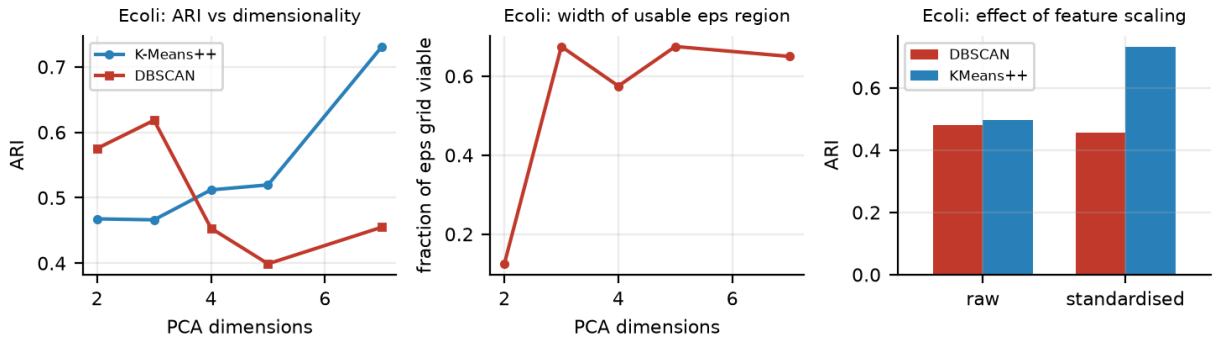
Figure 7: Ablations C and D on D4. Left: ARI against the number of principal components; DBSCAN leads at 2 and 3, K-Means++ from 4. Centre: share of the \varepsilon grid that gives at least 2 clusters with under 50% noise. Right: standardisation helps K-Means++ (0.497 to 0.731) and not DBSCAN (0.481 to 0.455). Cause: K-means depends on feature scale, and a density threshold weakens as dimensions are added.
