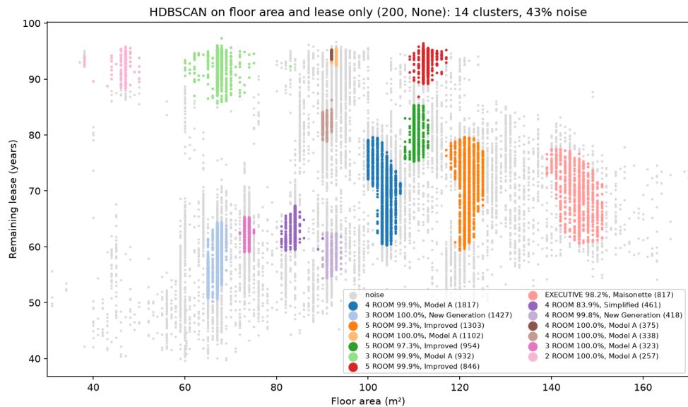
Figure 9: D8, success of HDBSCAN on floor area and remaining lease only ( min_cluster_size 200; grey: noise). Each cluster is one standard flat design; the legend gives its main flat type and model. Cause of success: fixed building plans create real dense spots in these two features.
