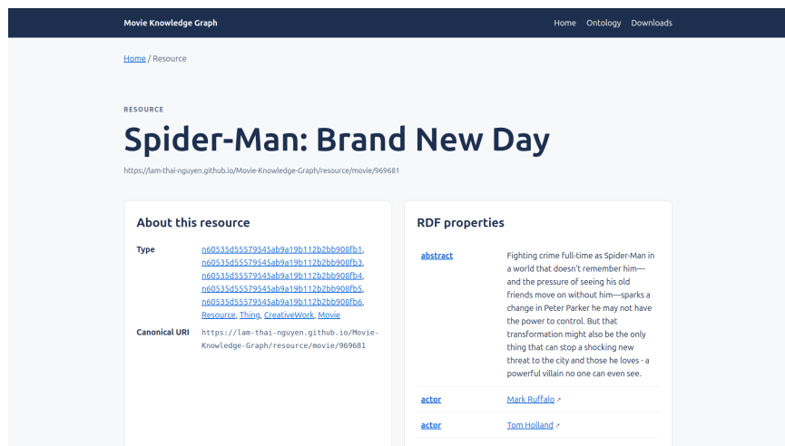
Figure 5: Representative generated resource page with its canonical URI and RDF properties.
