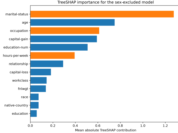
Figure 4: Mean absolute TreeSHAP contributions using the sex-excluded model. Orange bars indicate candidate proxies, while blue bars are not selected.
