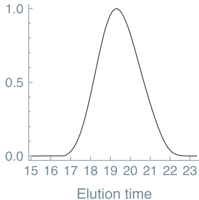
C: Poly(styrene-co-1-octene)
