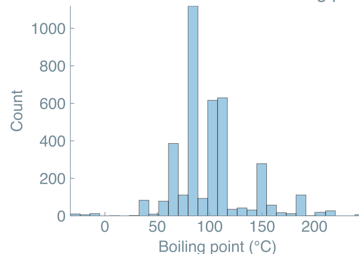
E Distribution of solvent boiling points
