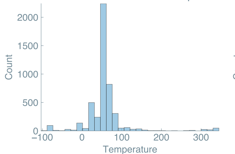
D Distribution of reaction temperatures
