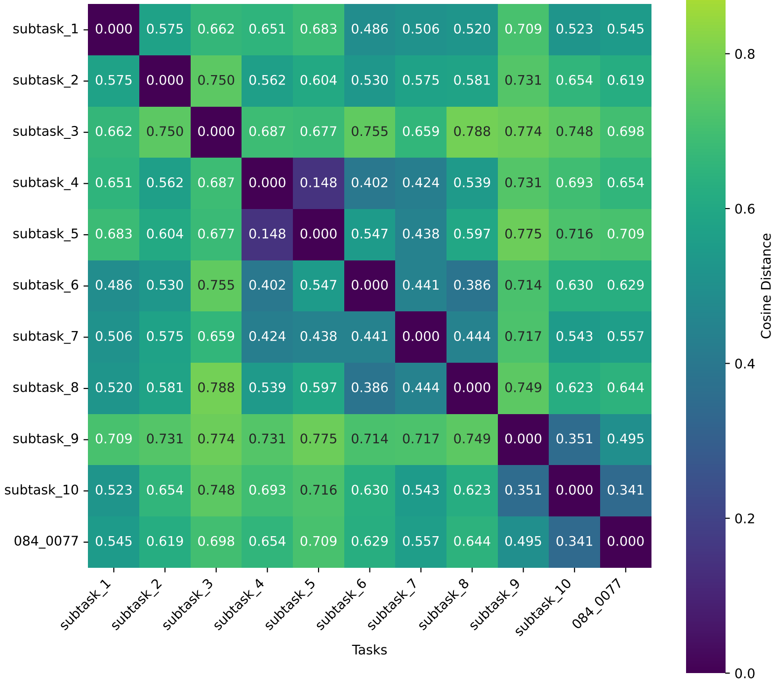
Tasks vs Tasks (Including Global Tasks) - Cosine Distance (L2 Normalized)
