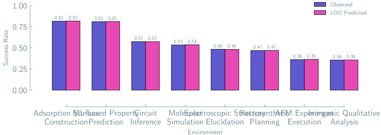
Environment-Level: LOO vs Observed
