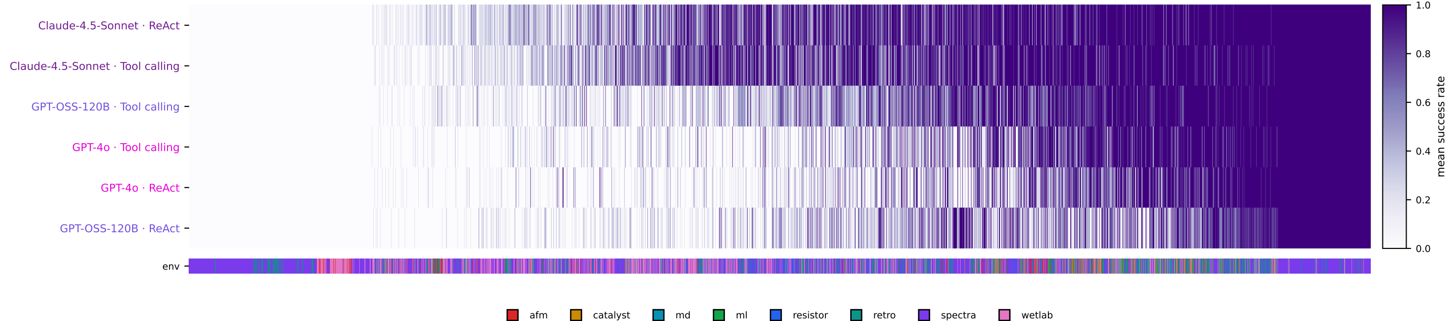
Sorted response matrix (6 model×scaffold subjects × 2703 items) rows: best subject top → worst bottom | columns: easiest item left → hardest right
