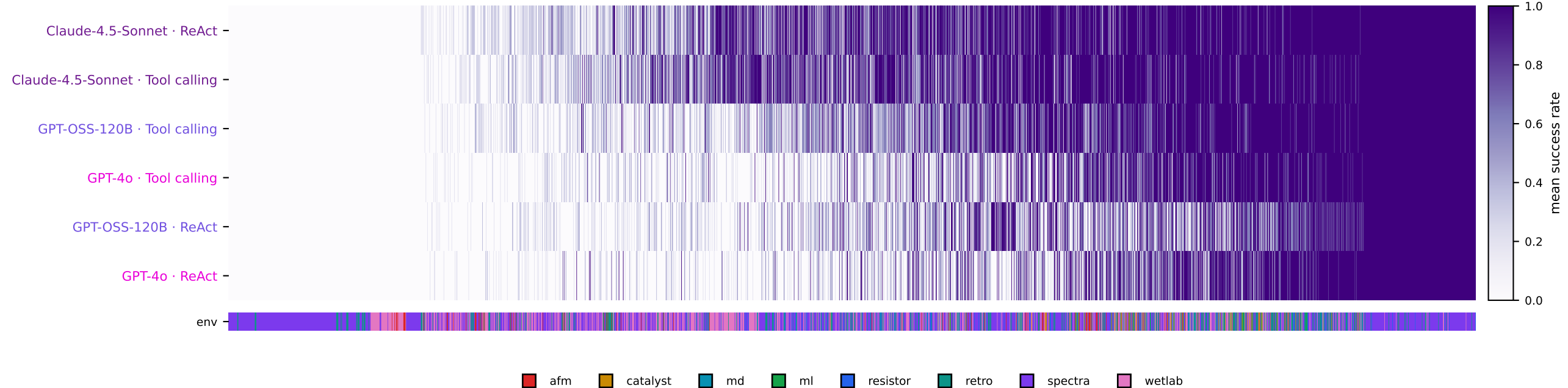
Sorted response matrix (6 model×scaffold subjects × 2358 items) rows: best subject top → worst bottom | columns: easiest item left → hardest right
