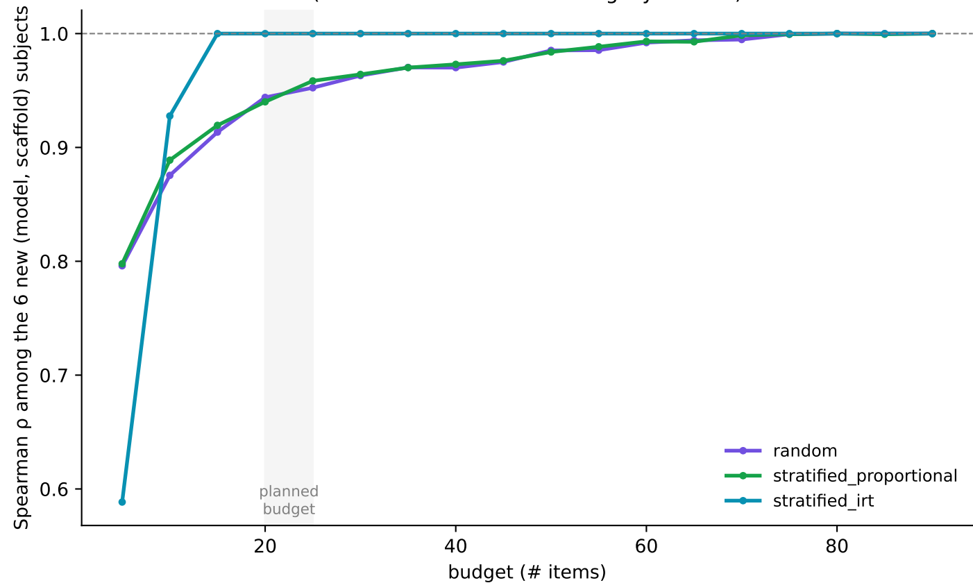
Ranking preservation on the 3 new test models (item set fit ONLY on the 3 legacy models)
