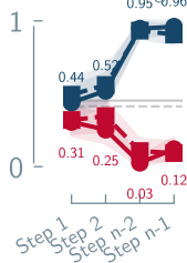
Retrosynthetic Planning
