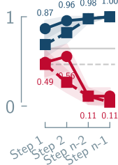
Circuit Inference
