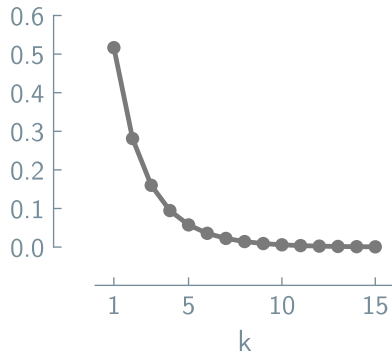
Molecular Simulation
