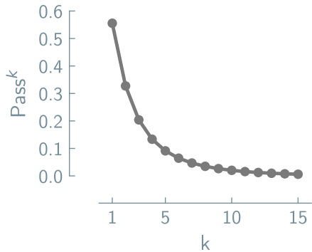
Circuit Inference
