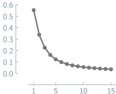
Molecular Simulation
