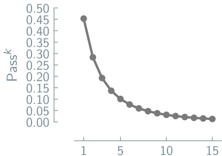
Circuit Inference
