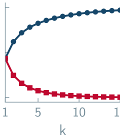
Retrosynthetic Planning
