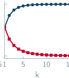
Circuit Inference
