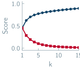
Spectroscopic Structure Elucidation
