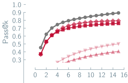
Spectroscopic Structure Elucidation
