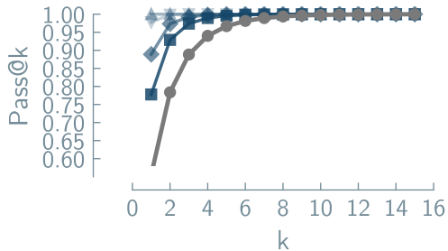
Circuit Inference
