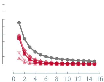
Molecular Simulation
