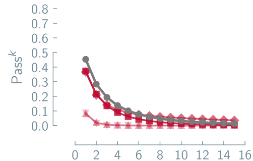
Circuit Inference
