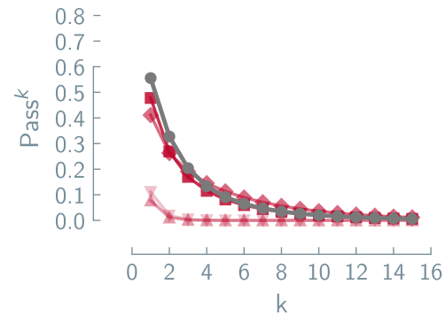
Circuit Inference
