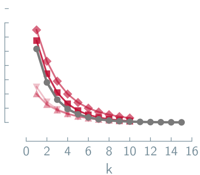
Molecular Simulation
