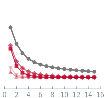
Molecular Simulation
