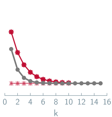
Molecular Simulation
