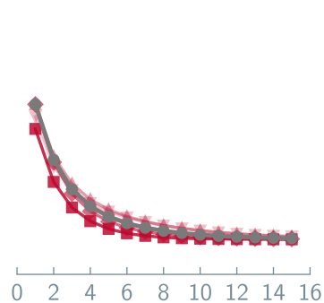
Retrosynthetic Planning
