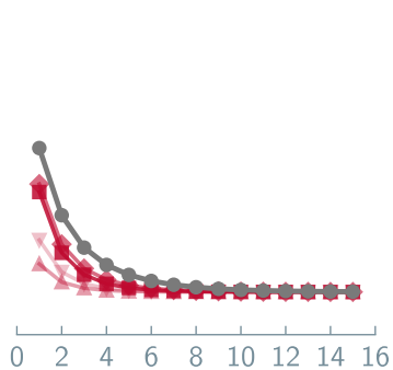
Molecular Simulation
