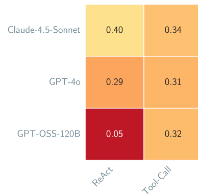
Retro- synthesis
