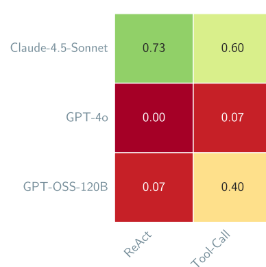
Retro- synthesis
