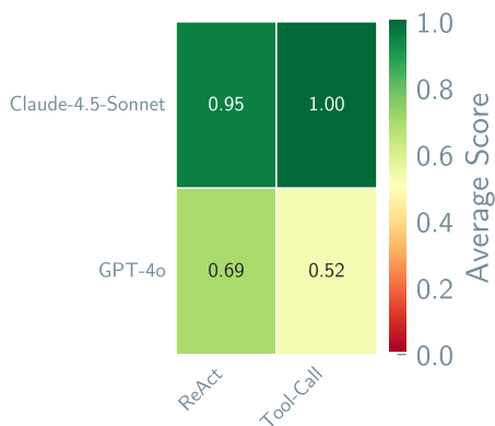
Machine Learning
