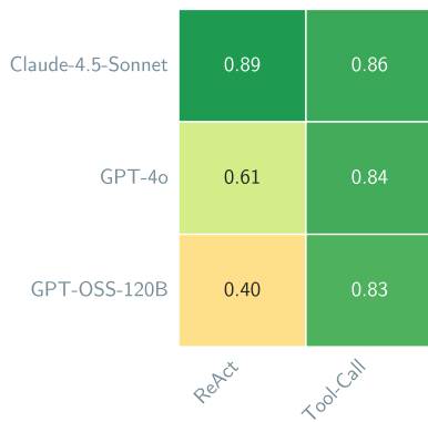
Machine Learning
