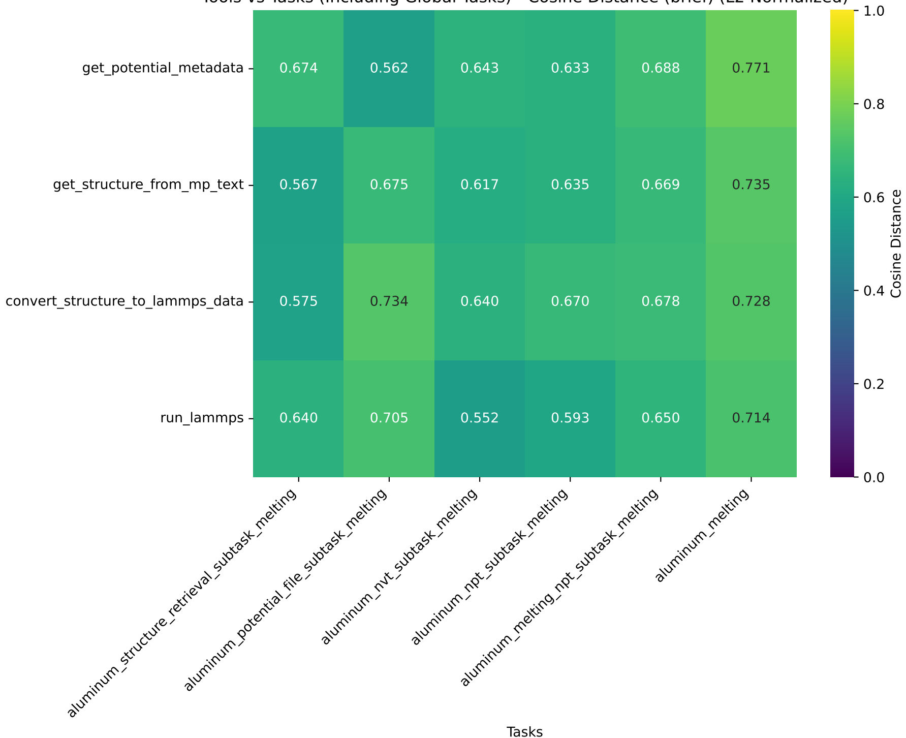
Tools vs Tasks (Including Global Tasks) - Cosine Distance (brief) (L2 Normalized)
